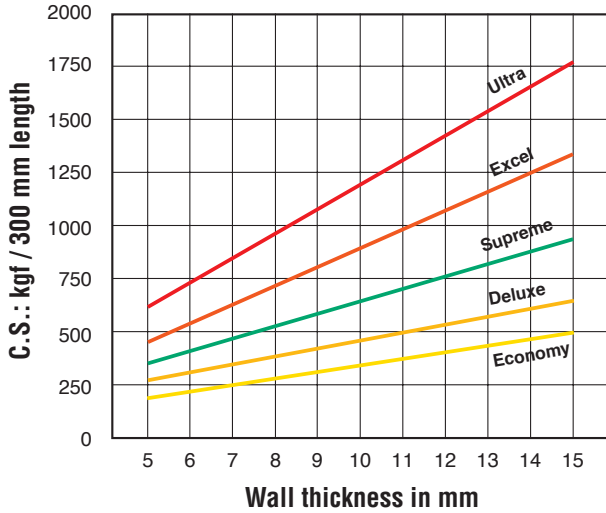
Flat Compression Strength of Film Cores for dia. 76.20 mm
