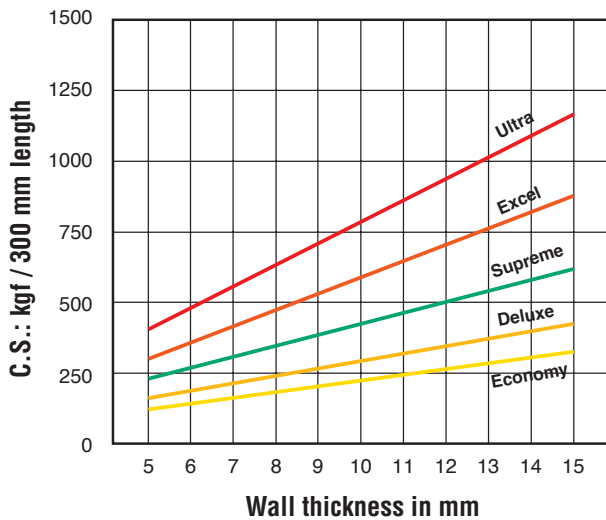
Flat Compression Strength of Film Cores for dia. 152.40 mm
